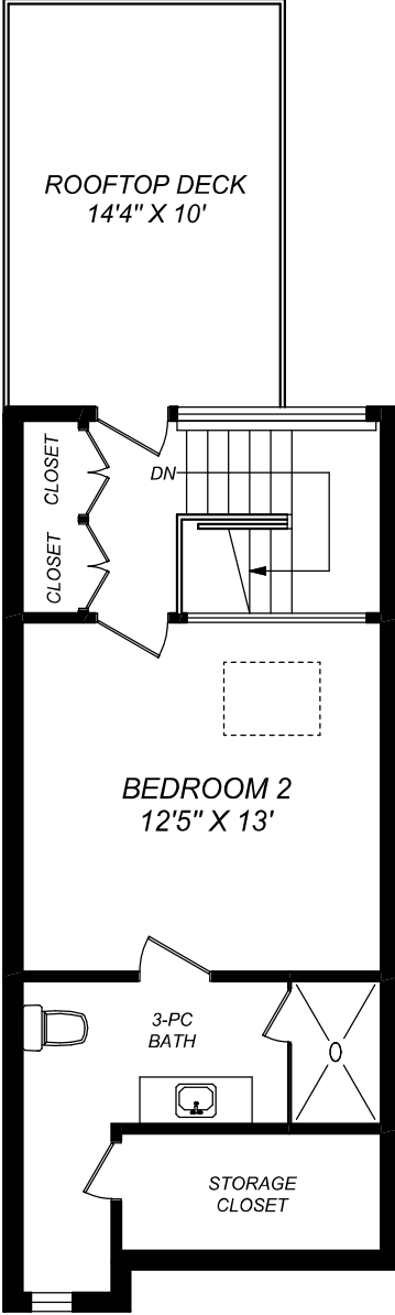
THIRD FLOOR 382 SQUARE FEET (VAULTED CEILING)
