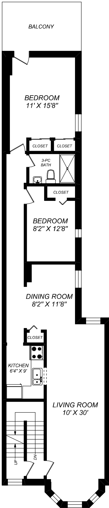
SECOND FLOOR 1116 SQUARE FEET (CEILING HEIGHT : 9'-3")
